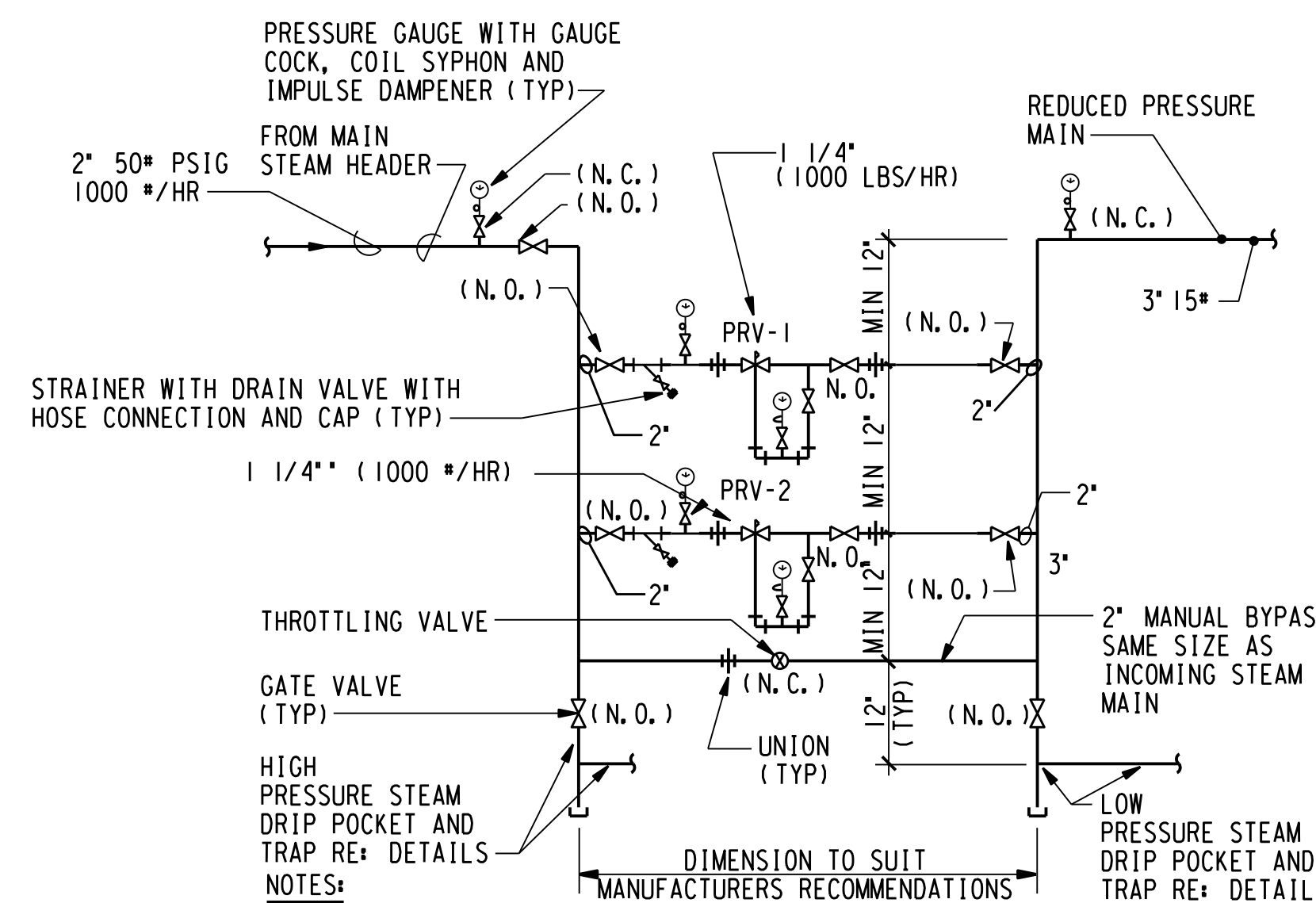
05 TYPICAL SINGLE STAGE STEAM PRESSURE REDUCING STATION NOT TO SCALE
